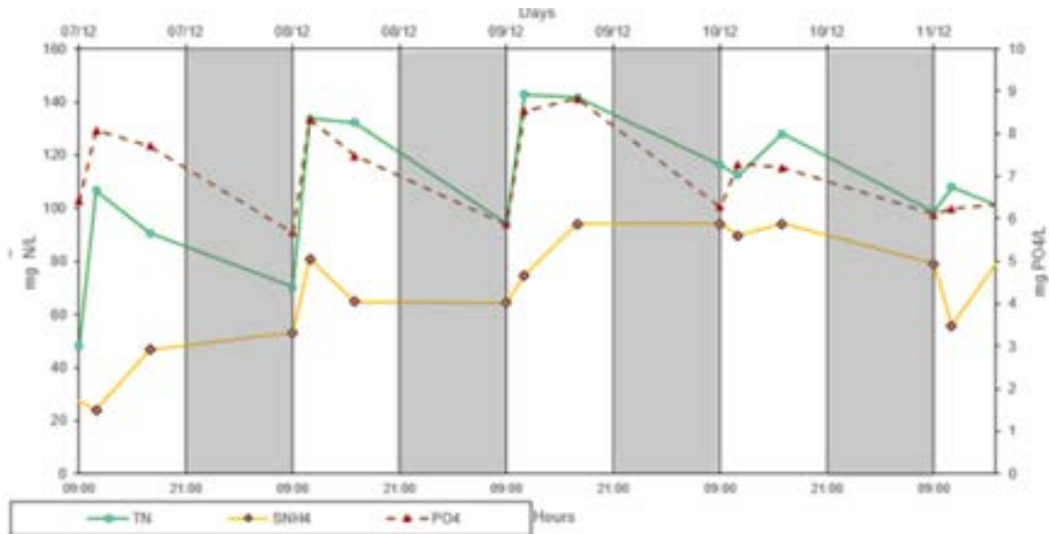
Figure 38 Evolution of total nitrogen (TN) ammonium (SNH 4 ) and Phosphate (PO 4 ) in the raceway reactor in the second week of operations in the phase 2
