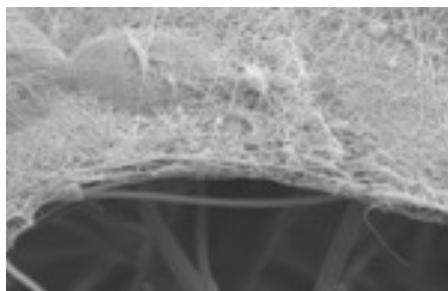
Figure 55. SEM picture of the NY6 nanocomposite membranes.
