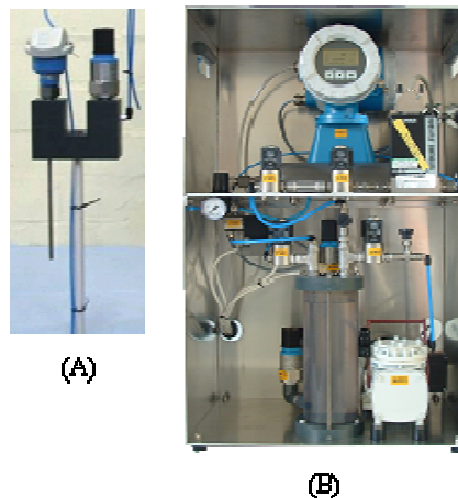
Figure 7. MBR-VFM set-up (A= sensor ; B= measuring device)
