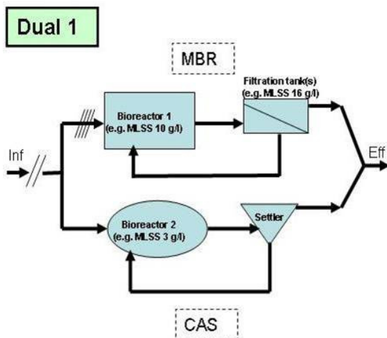
Figure 30. Dual 1 configuration
