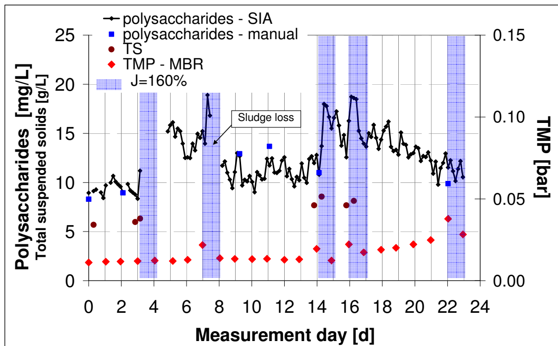
Figure 12. Variation of PS concentration in sludge filtrate of MBR measured continuously during simulation of inflow peaks (from 23rd March to 15th April 2009).
