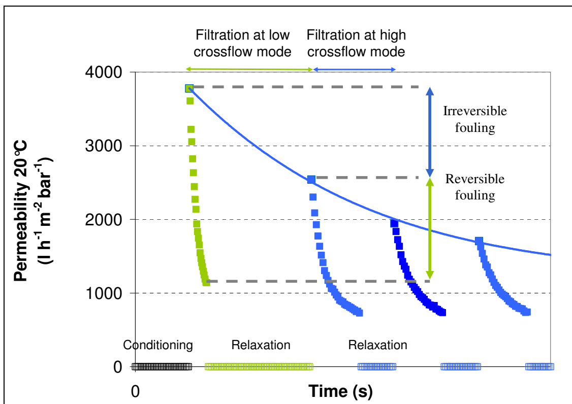
Figure 8. Schematic representation of MBR-VFM measurement protocol.
