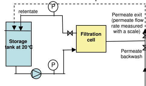
Figure 15. Pilot diagram to foul two flat sheet membranes with sludge supernatant
