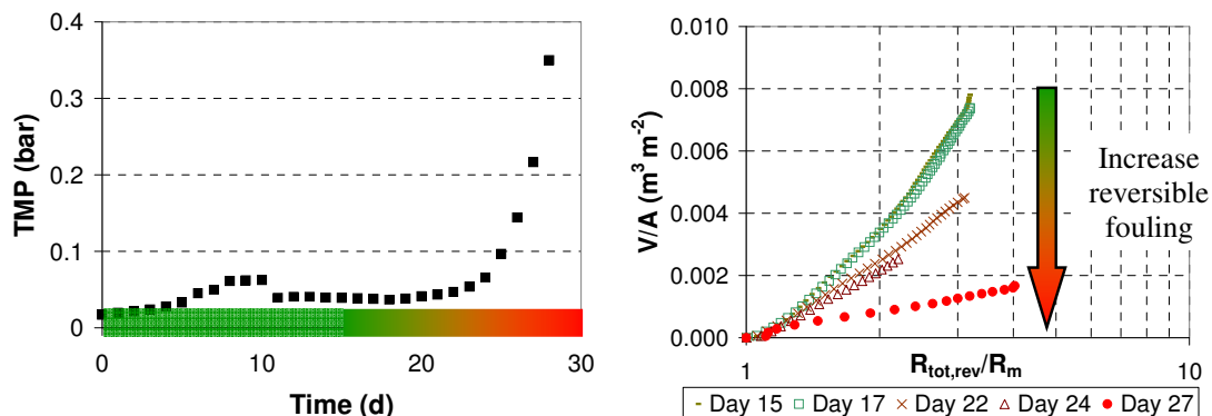
Figure 9. Evolution in on-line TMP measurement and reversible fouling fingerprints for a lab-scale MBR. V/A: m 3 of permeate per m 2 of membrane, R tot,rev /R m : ratio of total reversible fouling resistance and membrane resistance.
