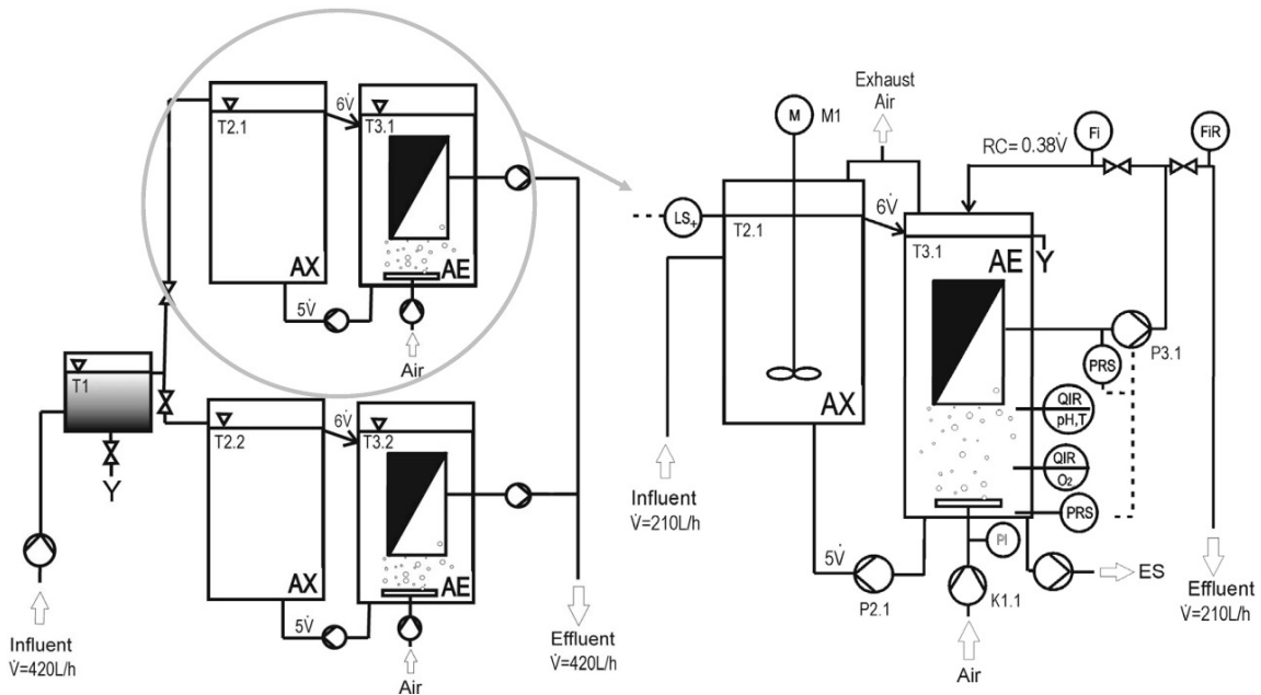
Figure 3. a) Set-up of the parallel pilot plants
