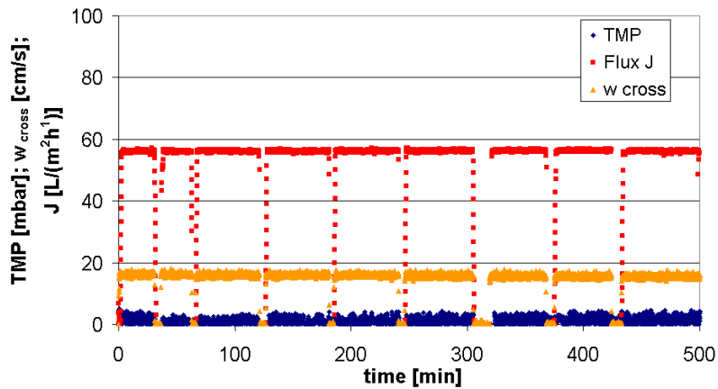
Figure 56. Stable operation if re-flocculation is applied
