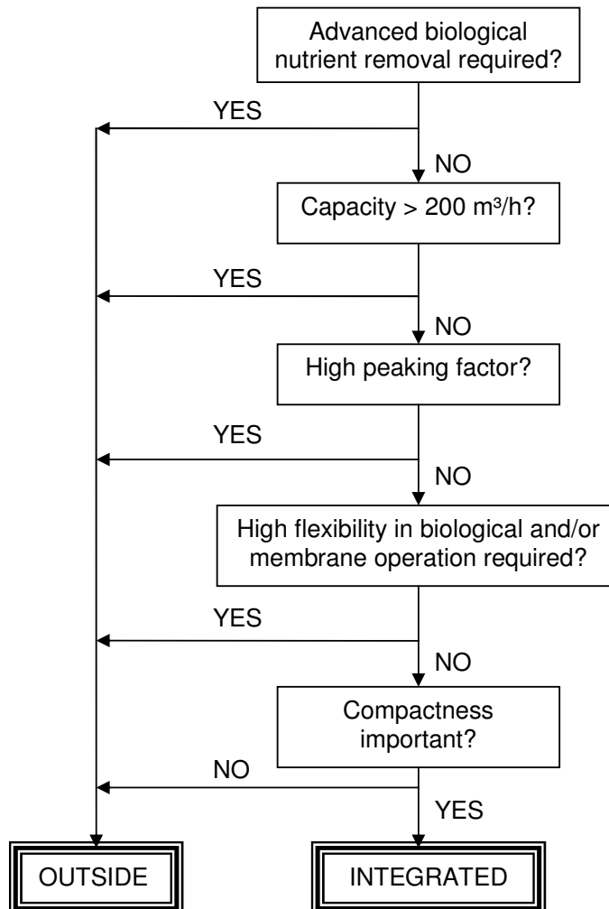
Figure 25. Decision tree for submerged MBR design.
