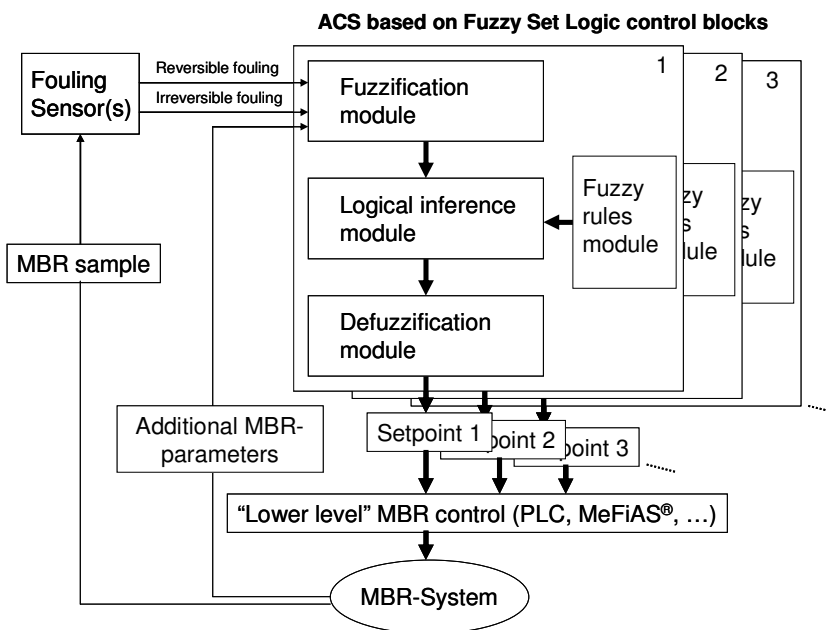
Figure 27. Advanced Control System (ACS) scheme
