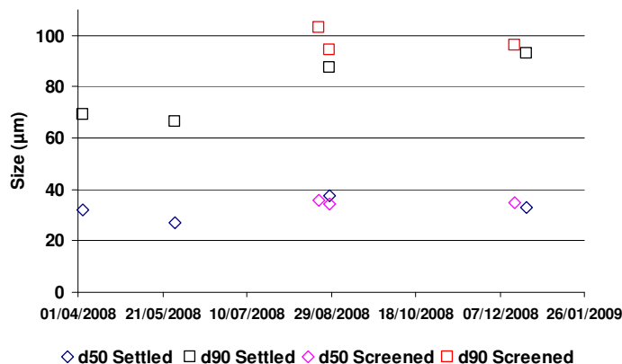
Figure 19. Floc size distribution comparison between settled and screened pilots
