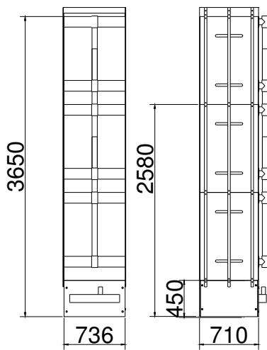
Figure 46. Design of the A3 triple deck module
