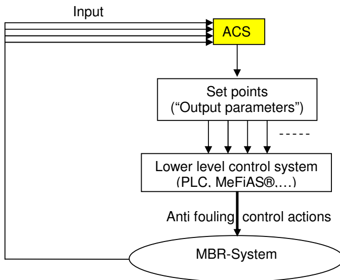
Figure 26. Concept of advanced control system (ACS) approach
