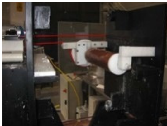
Figure 54. Picture of the electrospinning prototype designed and constructed by TTX
