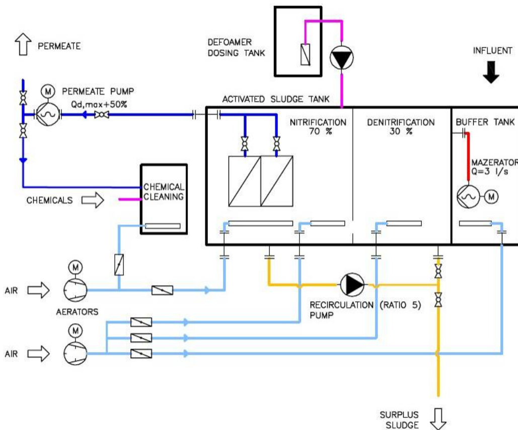
Figure 58. Flow diagram of containerised WWTP
