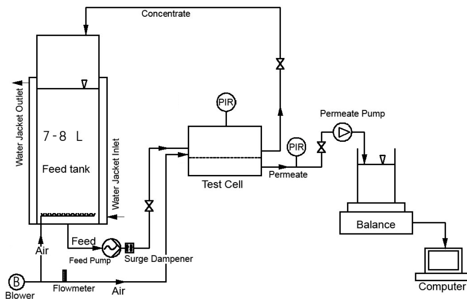
Figure 2. Flow sheet of the filtration test cell
