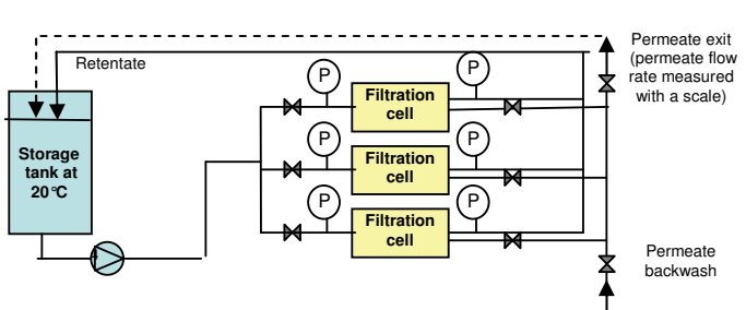
Figure 16. Pilot diagram to foul three hollow fibres bundles or FiSh modules with sludge supernatant
