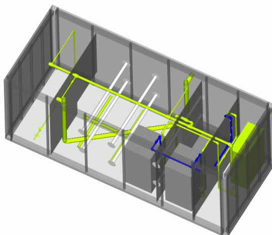
Figure 59. 3D picture of containerised system (200 pe)
